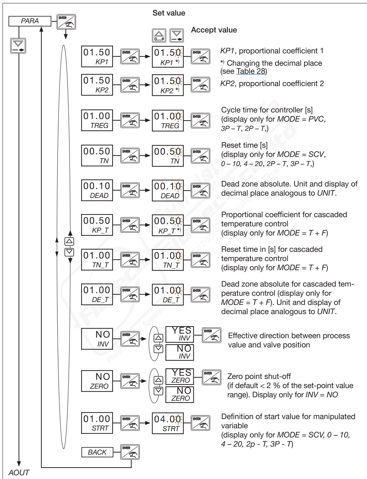
Figure 54: PARA; Adjusting the controller parameters
