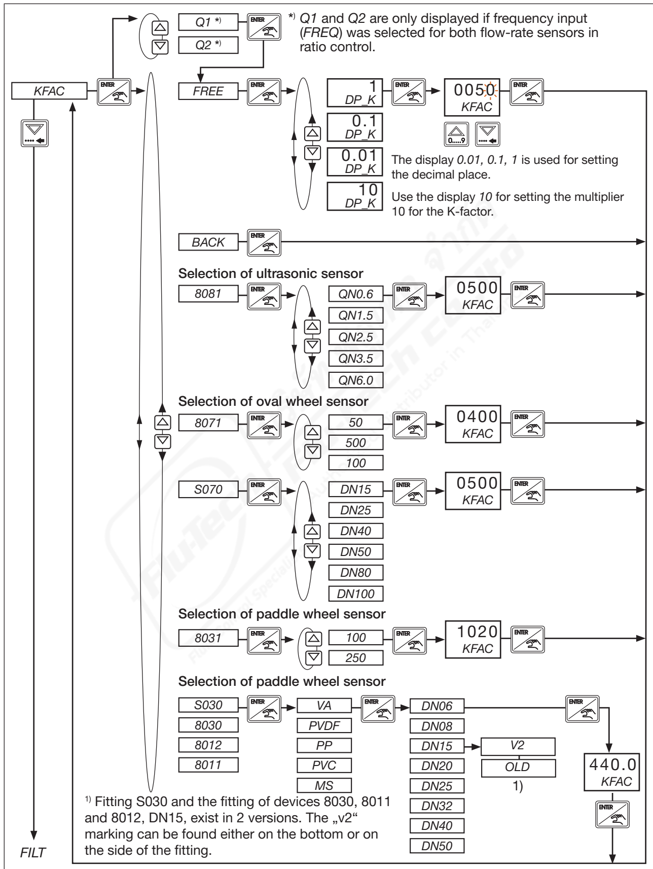
Figure 52: KFACT; entry of K-factor
