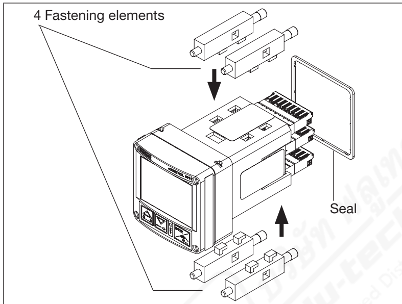
Figure 7: Installation elements
