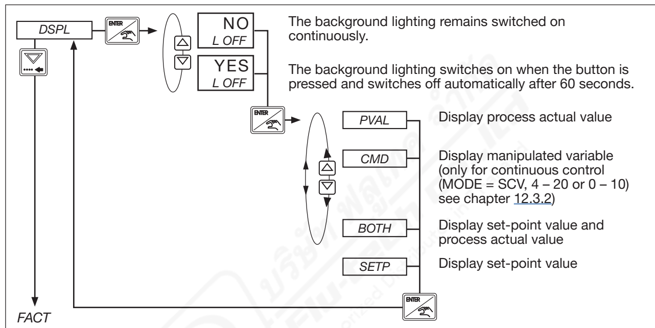
Figure 69: DSPL; Setting the display
