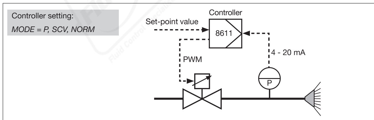
Figure 33: Pressure control using proportional valve
