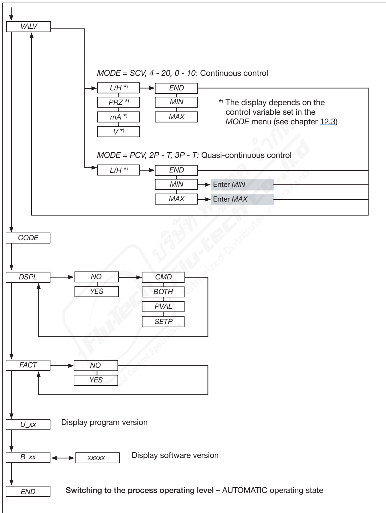
36 Figure 18: Operating structure of the configuration level - 6 of 6
