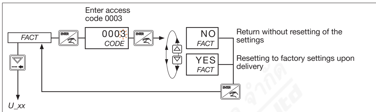
Figure 70: FACT; Reset to Factory Settings
