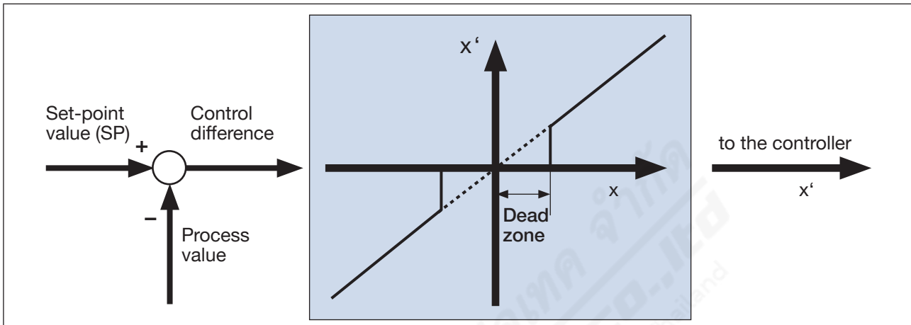
Figure 55: DEAD; Insensitivity range (dead zone)
