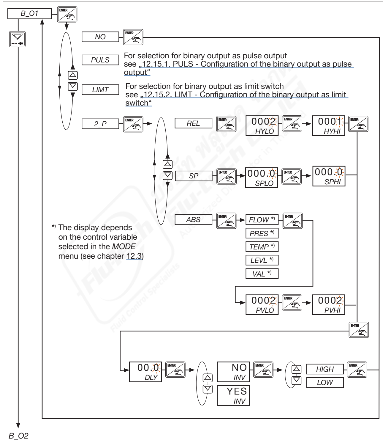
Figure 65: B_O1; Configuration of the binary output as 2-state control (2_P)
