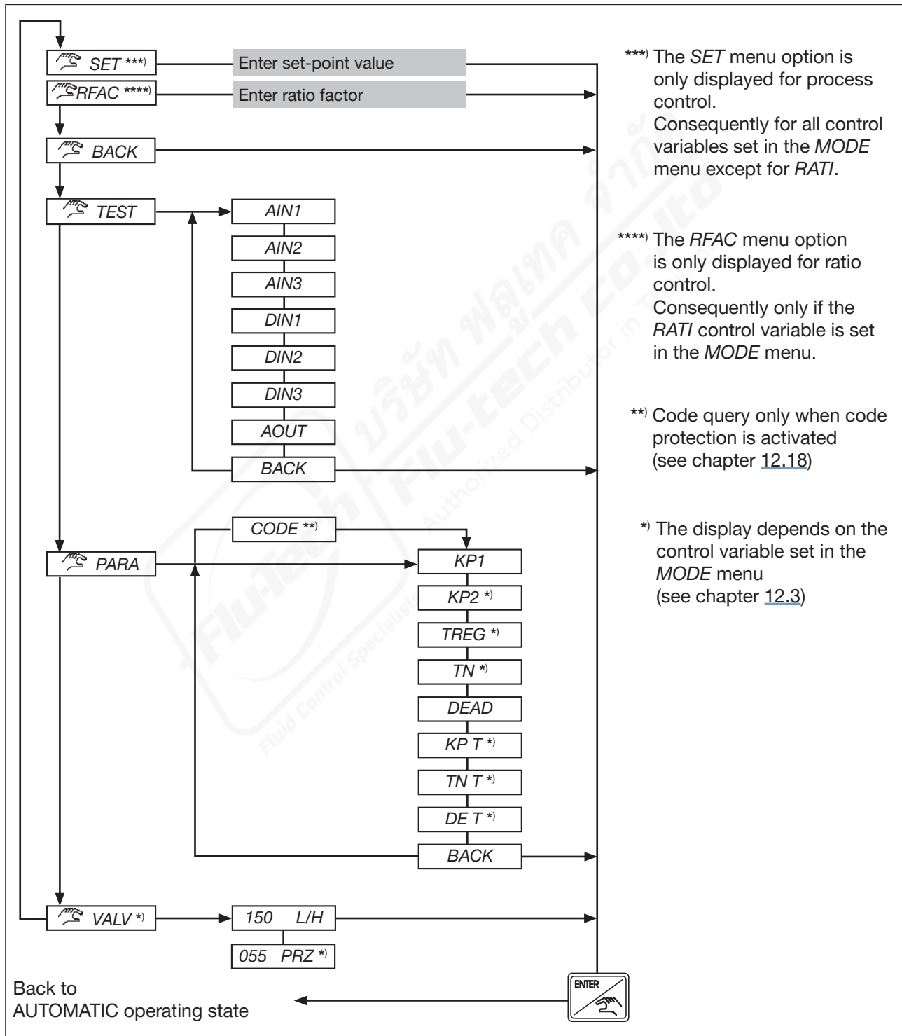
Figure 12: Operating structure of the process operating level in MANUAL operating state
