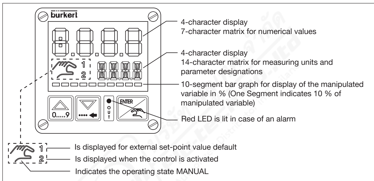
Figure 10: Display elements
