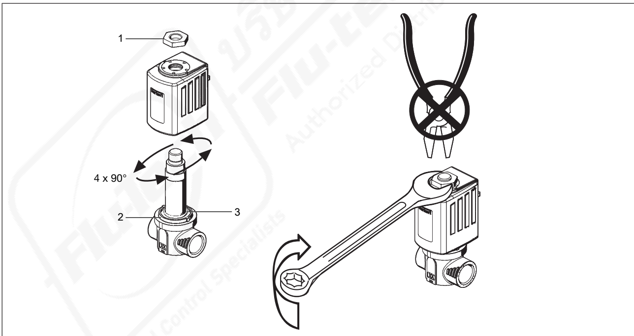
Fig. 13: Coil installation
