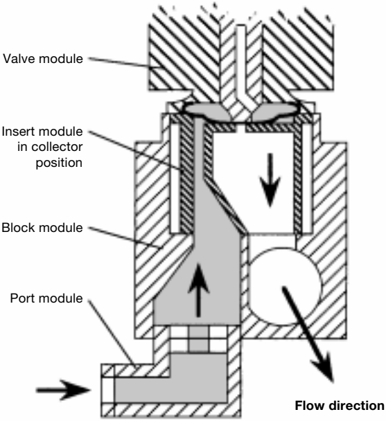
Collector mode (scheme):
