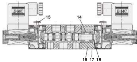
5/3 Solenoid Valve
