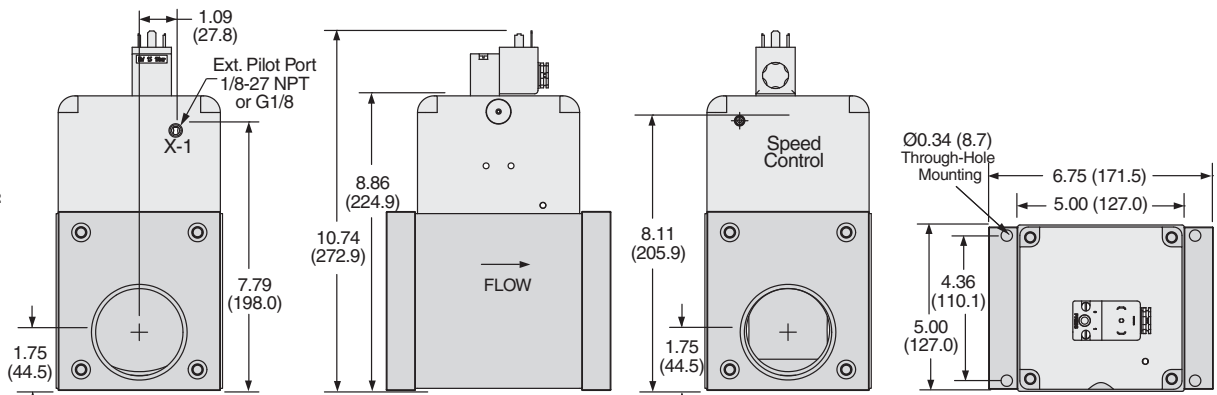
Port Size 2 & 2 1/2
